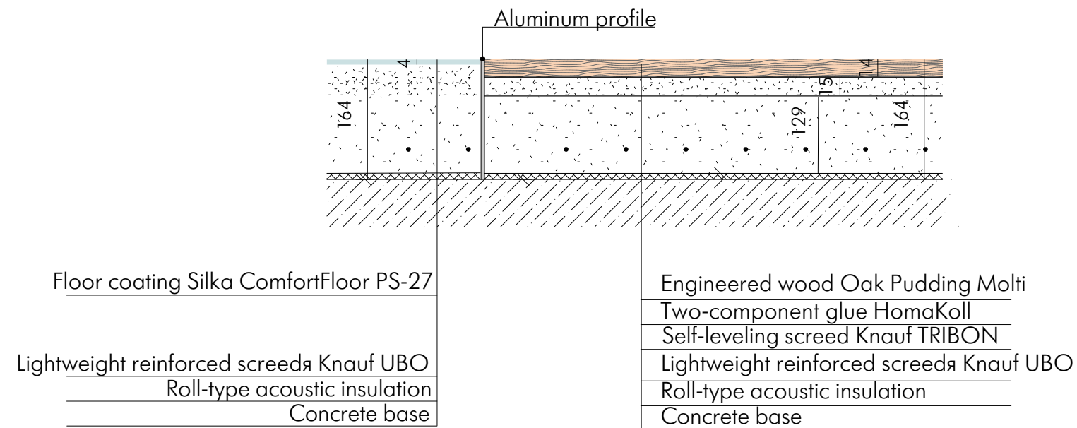
Detail B
