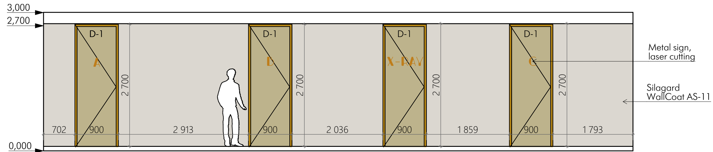
Wall E-F
