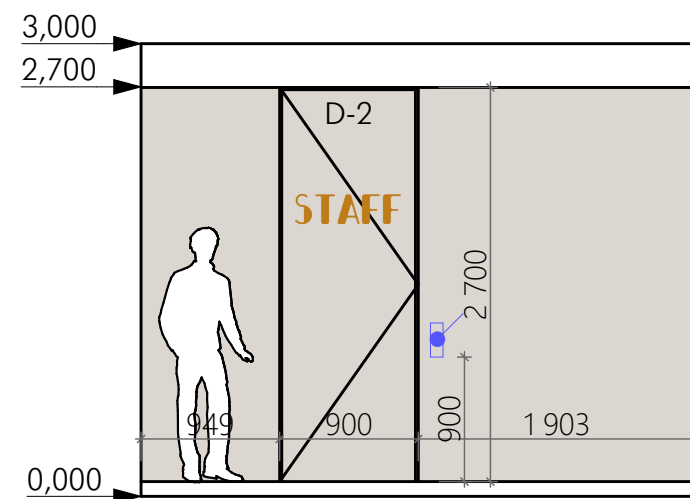
Wall G-K
