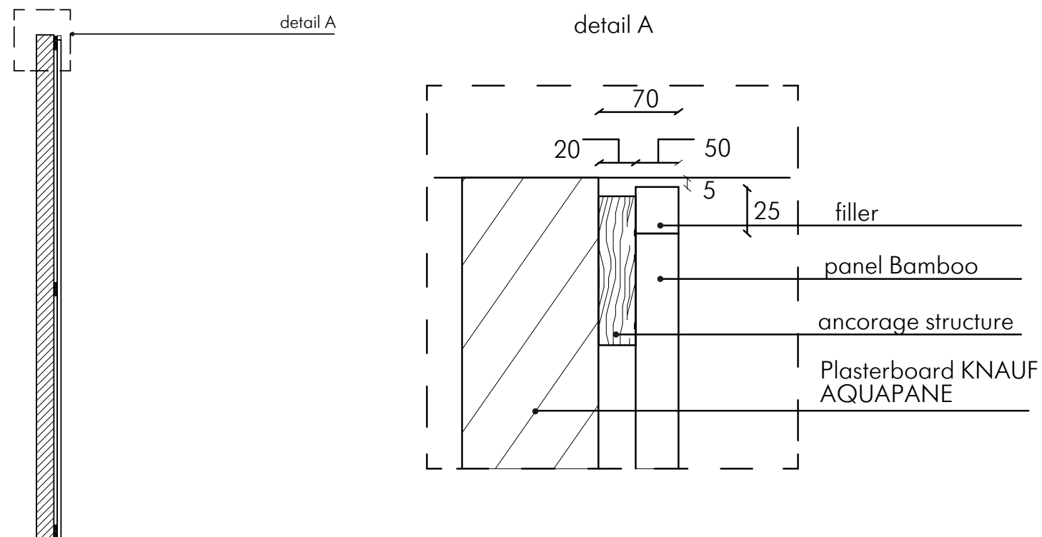
Detail A
