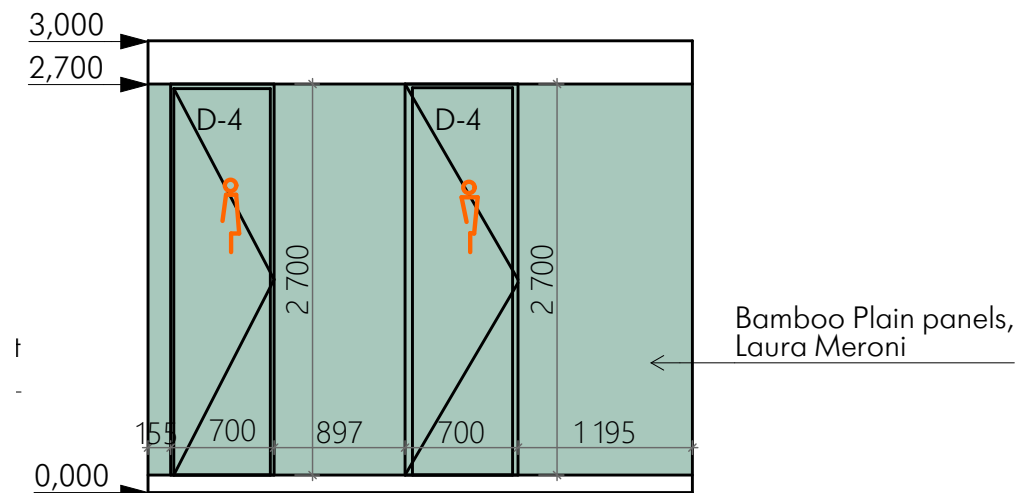
Wall O-P
